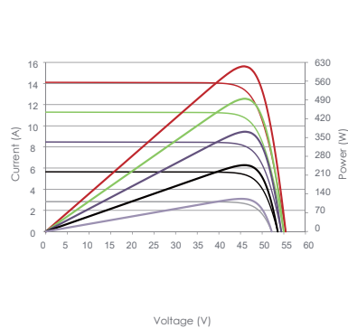
Current-Voltage & Power-Voltage Curves (615W)
